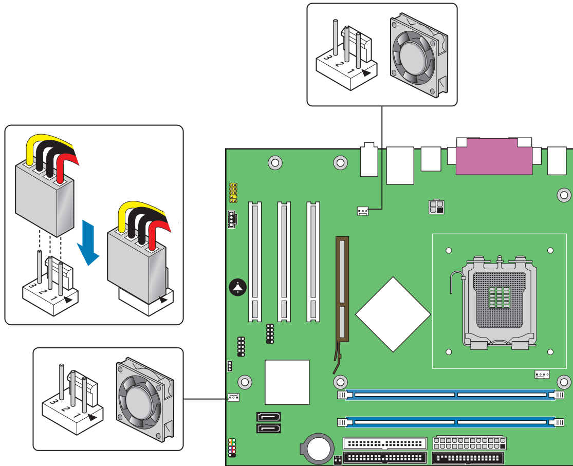
Figure 21. Location of Chassis Fan Headers
